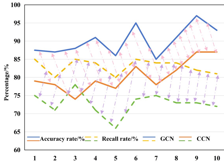
Figure 2 GCN and CNN clothing style contour recognition accuracy rate and recall rate
