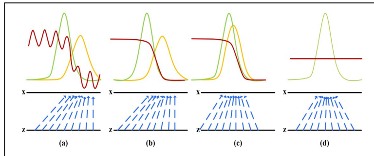
Figure 4 Dynamic changes of generator and discriminator during GAN training
